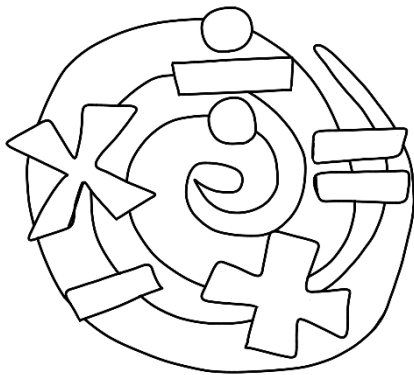
math
