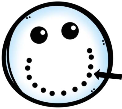
mouth CVC
